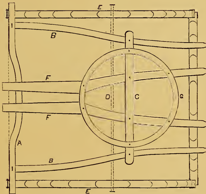
SECTIONAL CARRIAGE-PART FOR THE PEDDLER'S WAGON, ON PLATE 20.
